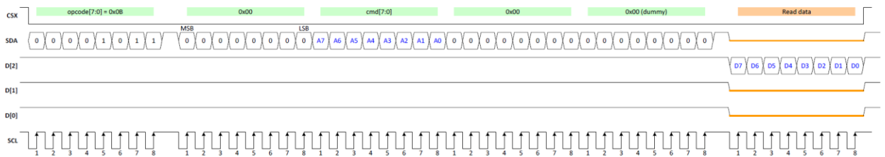
Figure 6-12: QSPI Read
