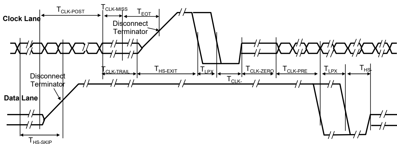
Switching the Clock Lane between Clock Transmission and LP mode
