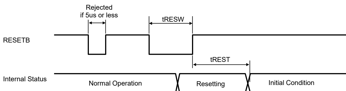
RESETB input timing
