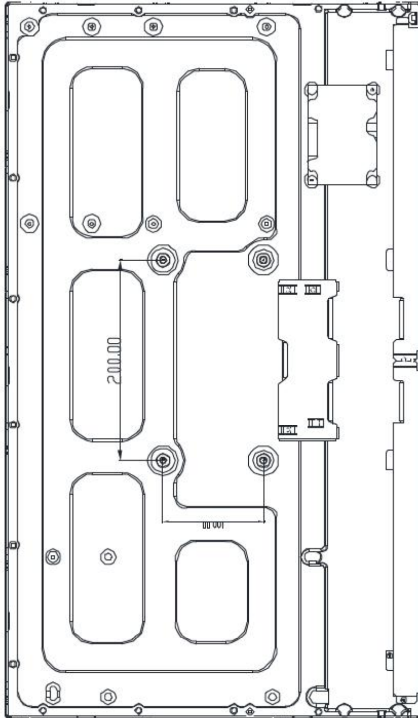
TFT-LCD Module Outline Dimensions(RearView) mm
