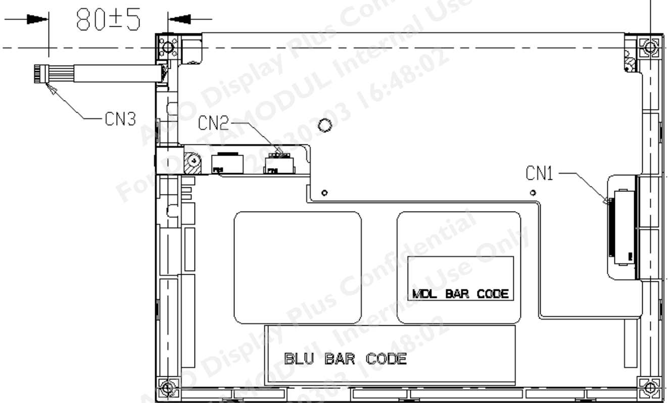
( Rear side of TFT-LCD )
