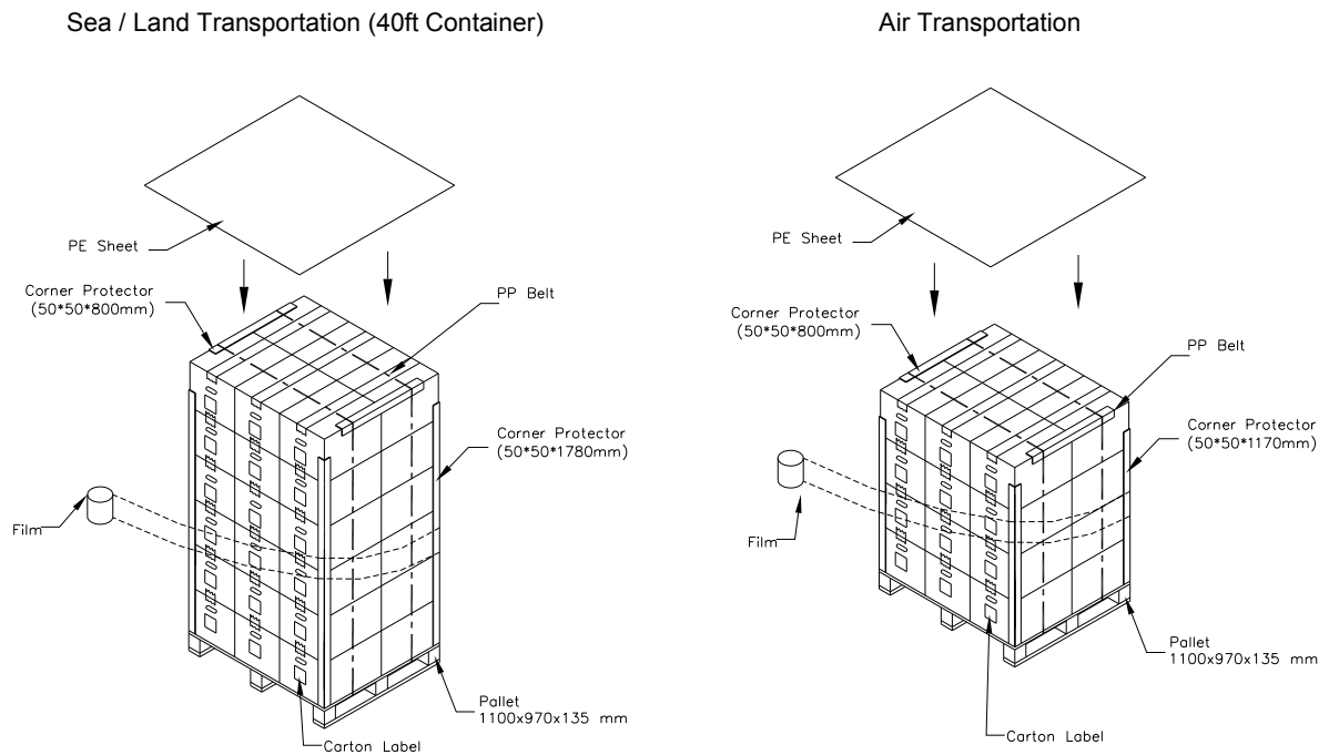
Figure. 9-2 Packing method
