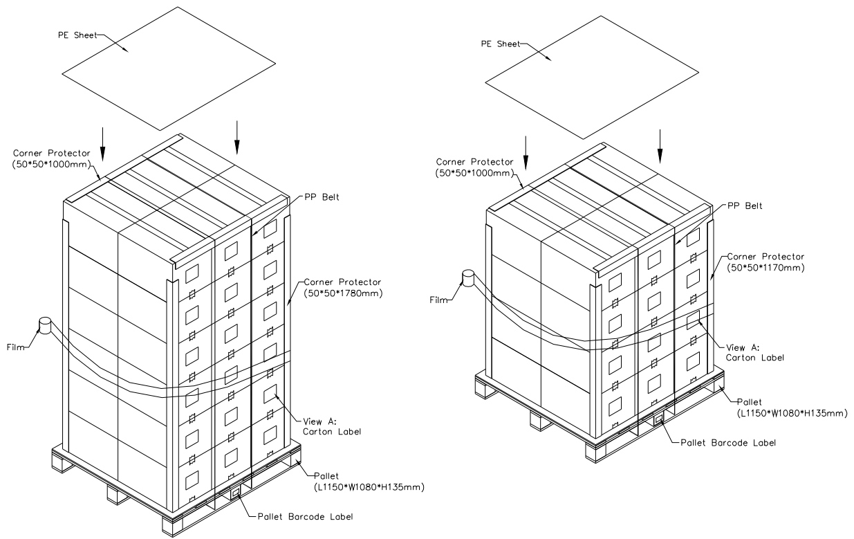
Figure. 9-2 Packing method
