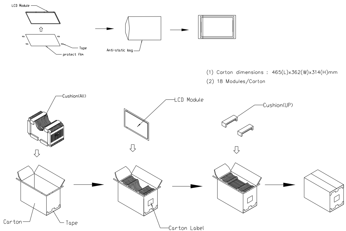
Figure. 9-1 Packing method
