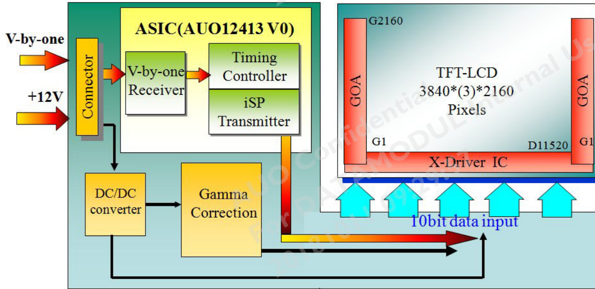
X PCB
