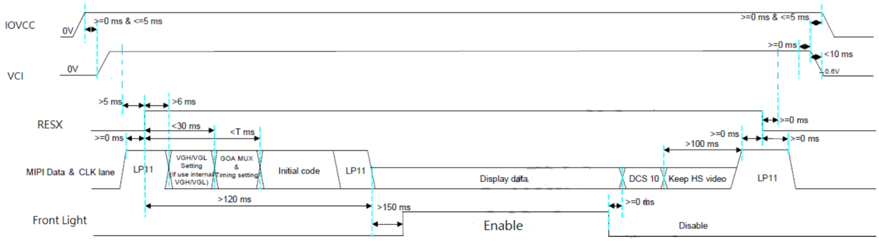
Power on/off sequence
