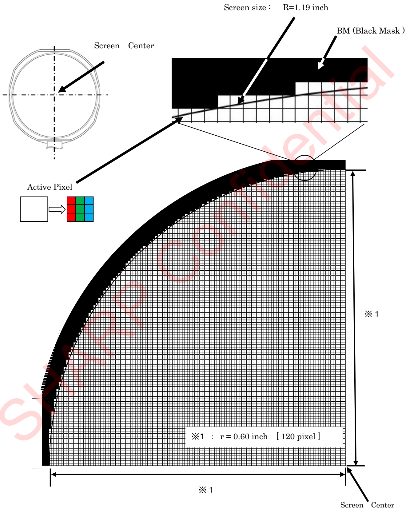
Figure 6-5-2 Data position 2
