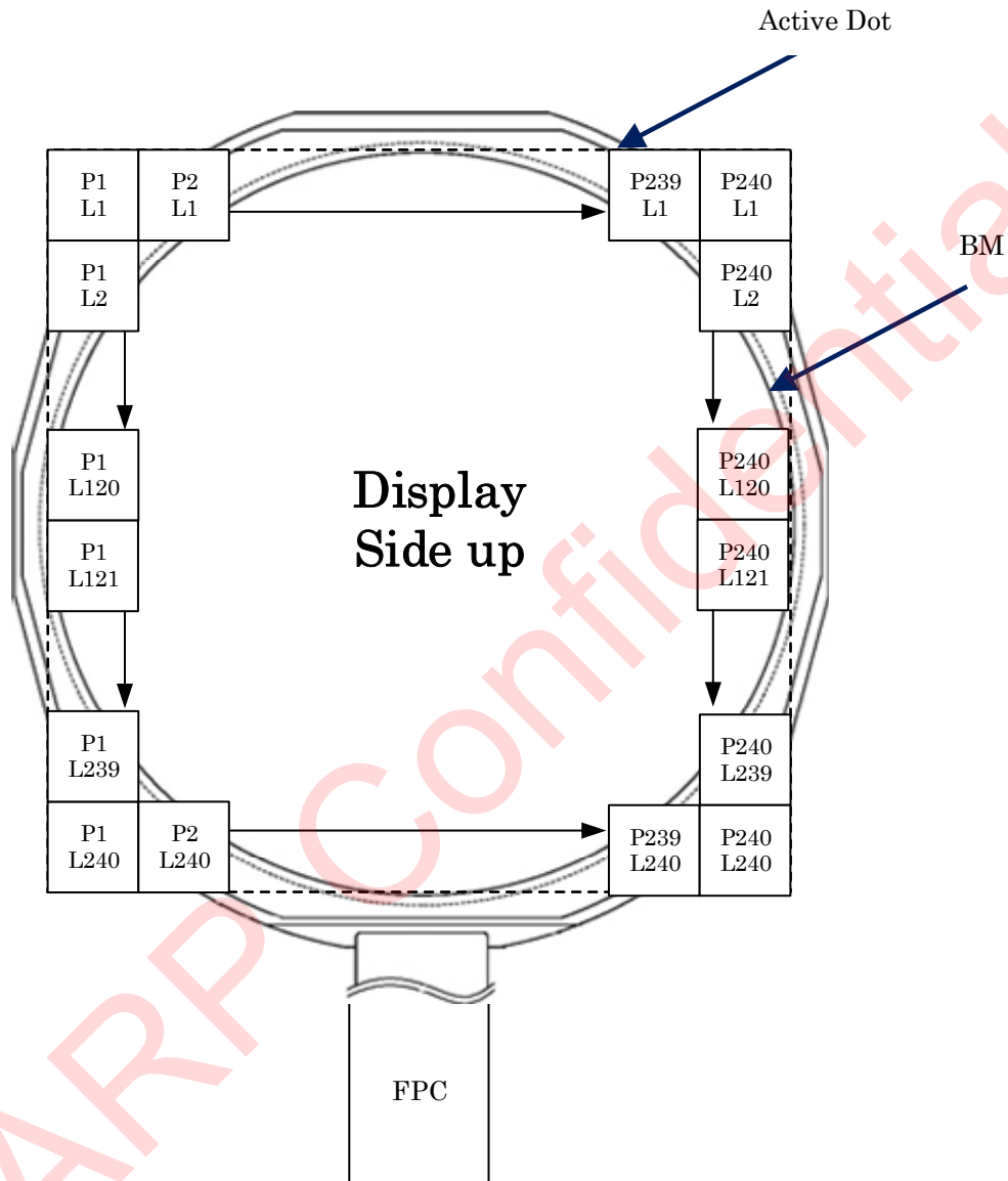
Figure 6-5-1 Data position 1
