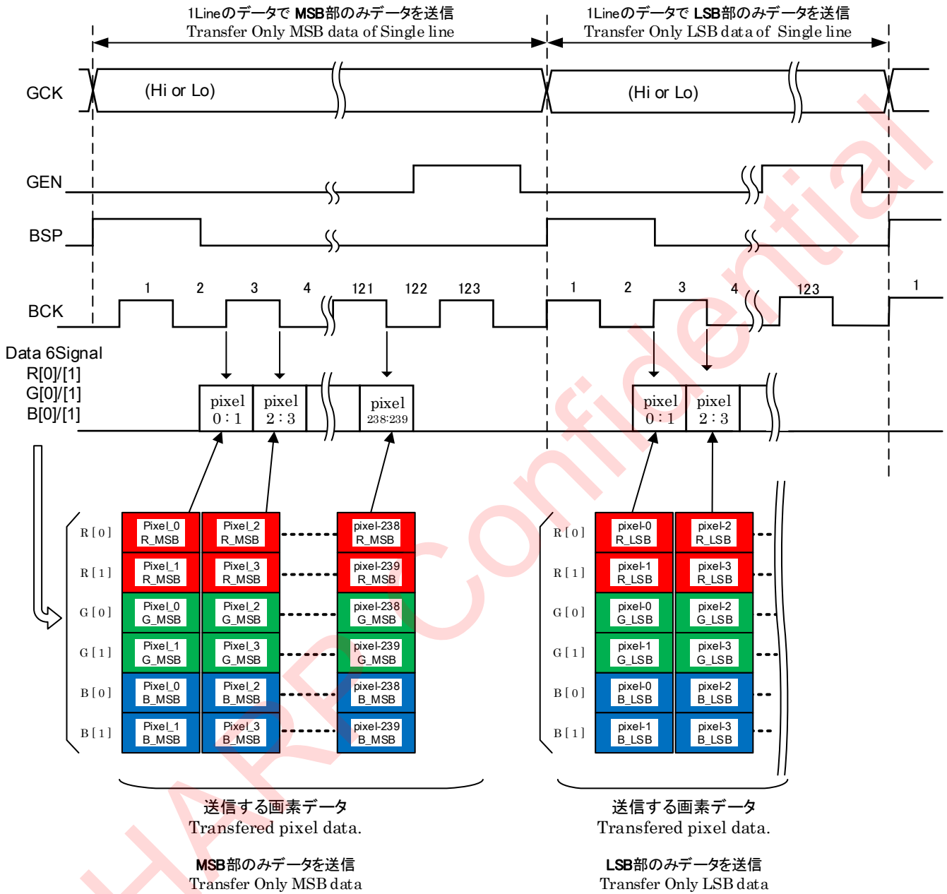
Figure 6-8-2 Horizontal timing
