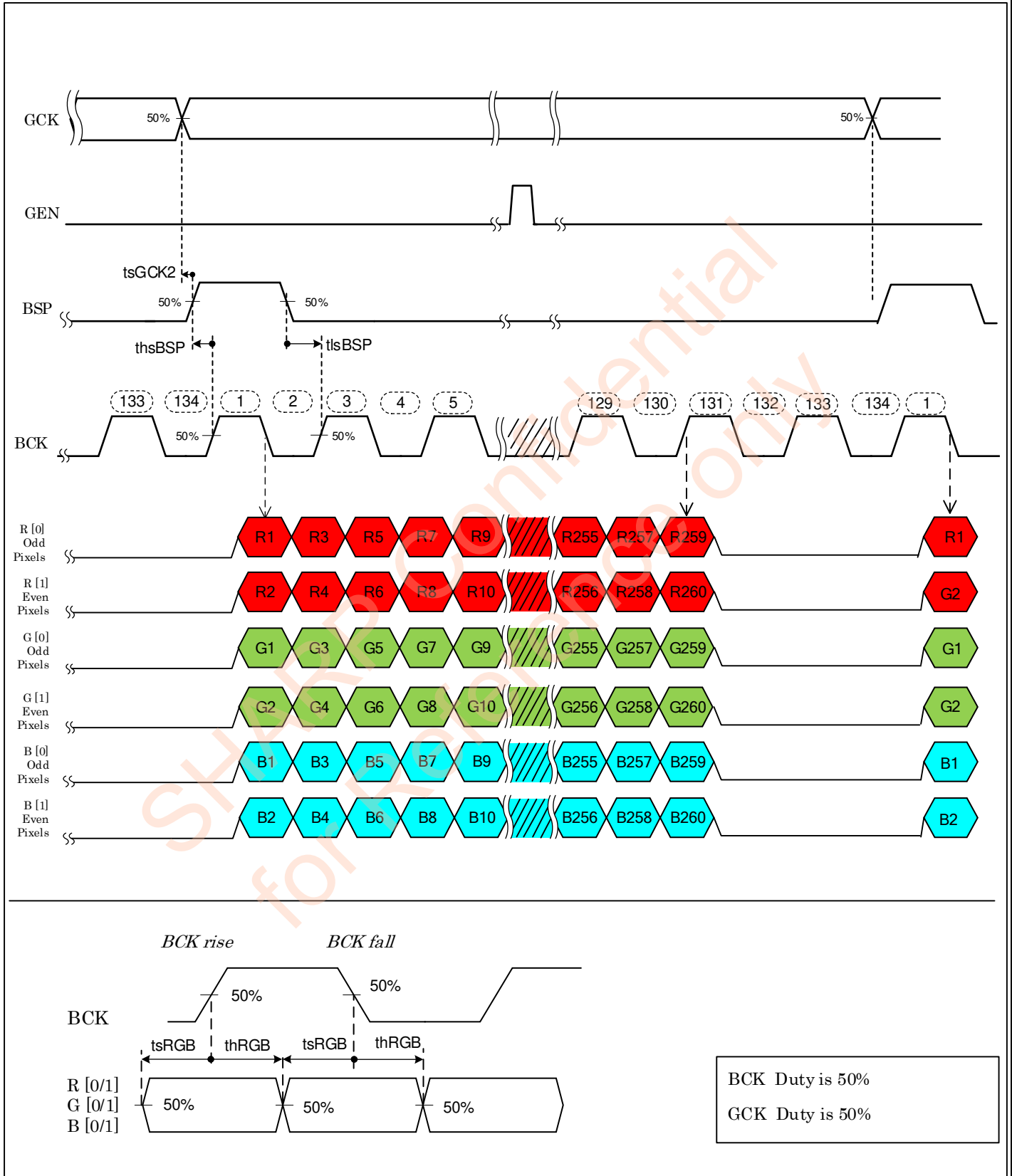
Figure 6-3-3 AC timing 3
