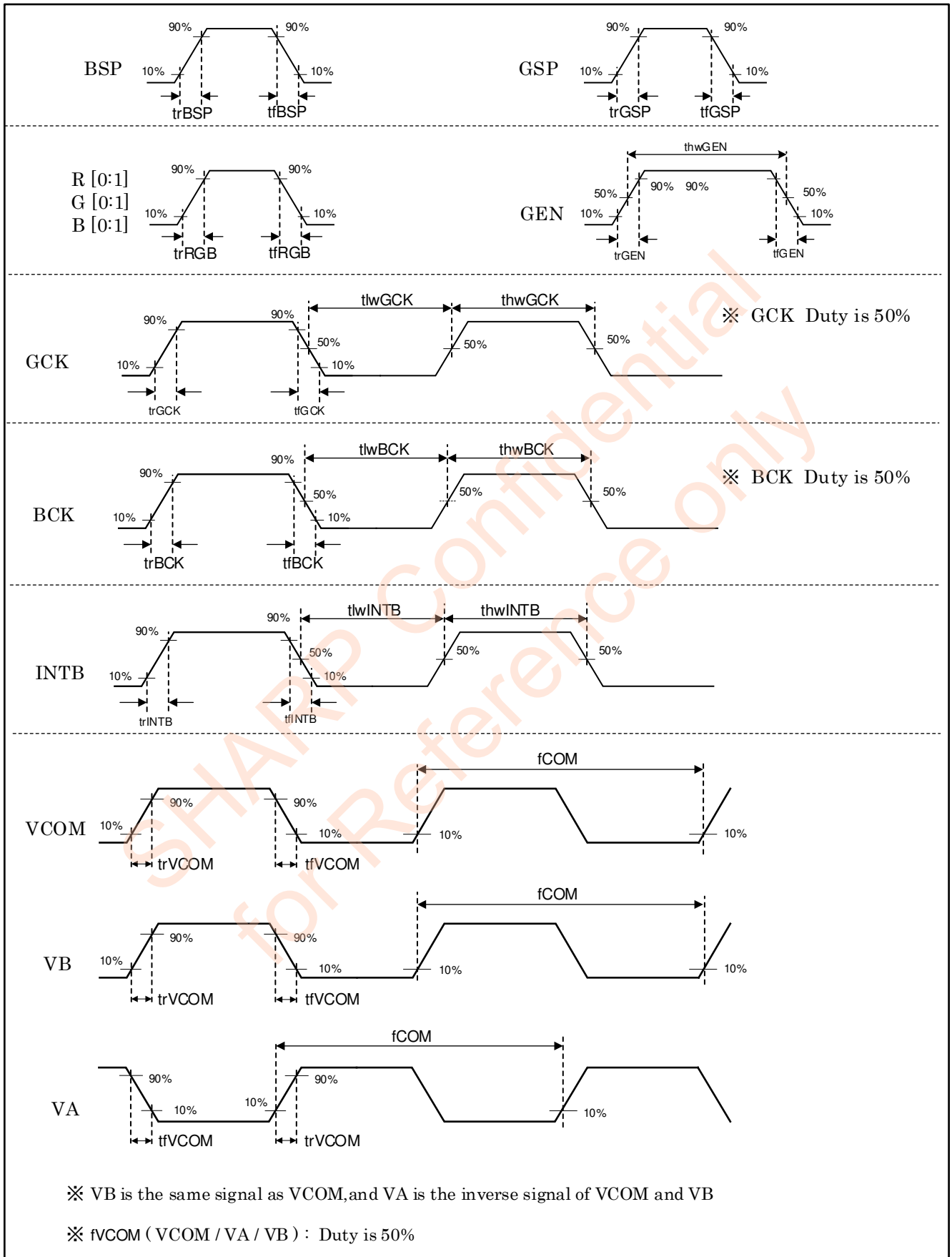
Figure 6-3-1 AC timing 1
