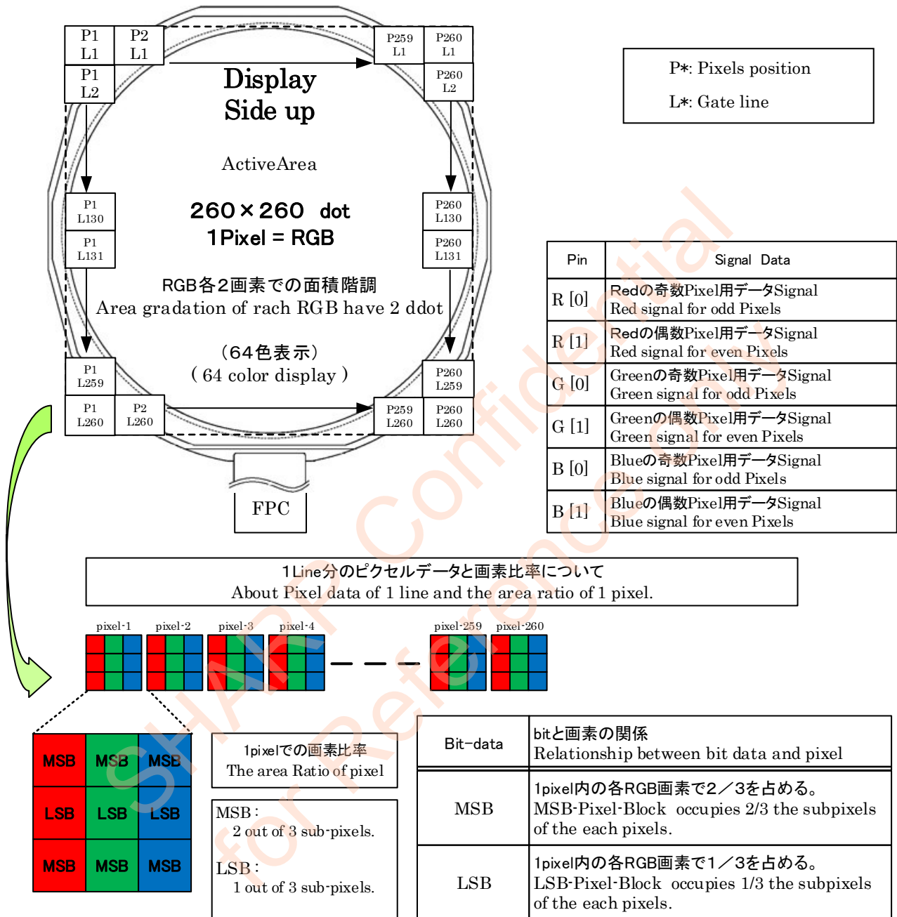
Figure 6-6-1 Data position 1
