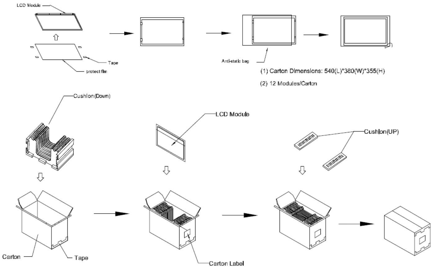
Figure. 8-1 Packing method
