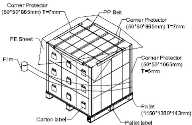
Figure. 8-2 Packing method
