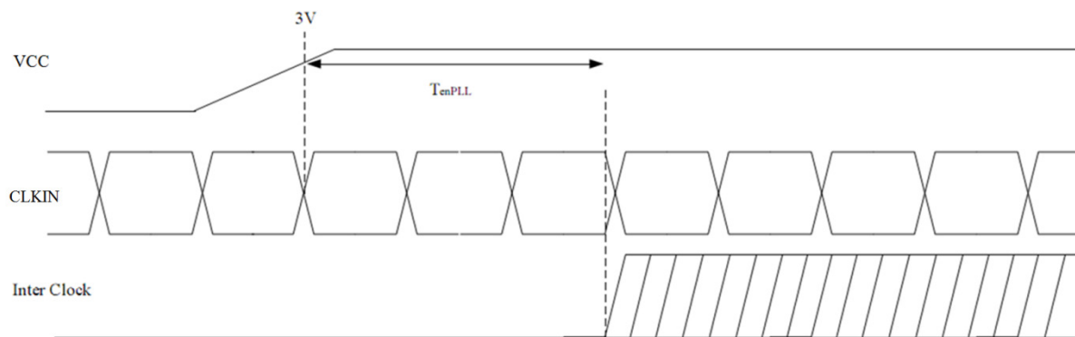
Figure 6.1.2 LVDS mode AC electrical characteristics 2
