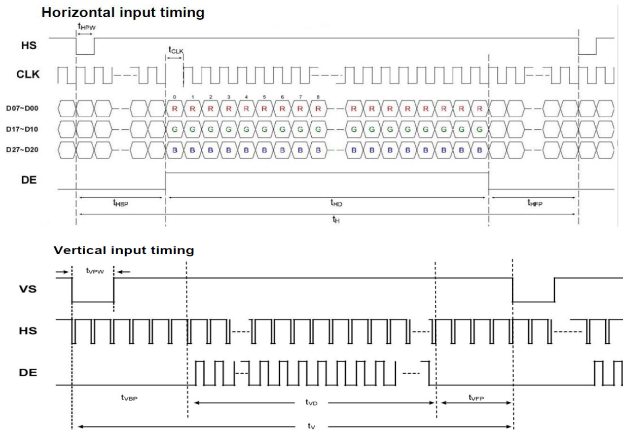
Figure 6.3.2 Input timing
