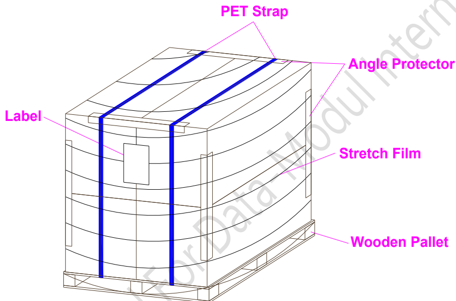
Single pallet packaging illustration
