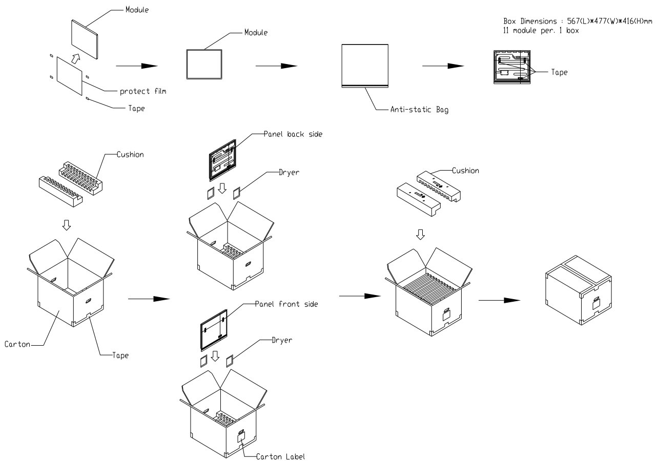
Figure. 7-1 Packing method
