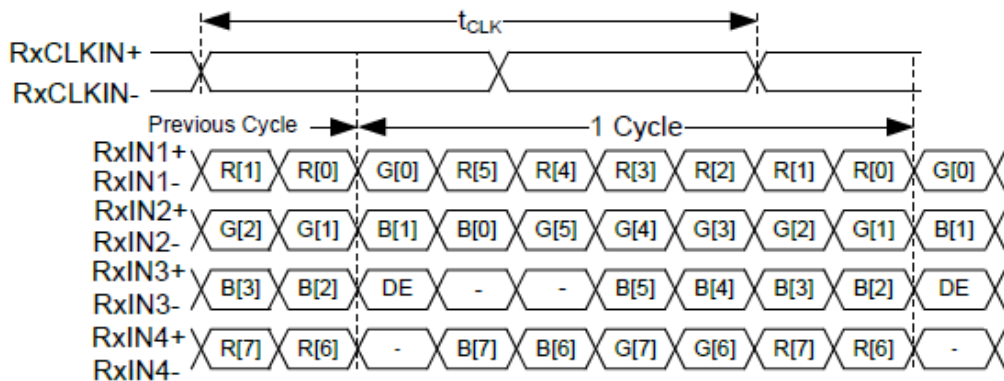
Figure6.2 LVDS input data mapping(VESA)
