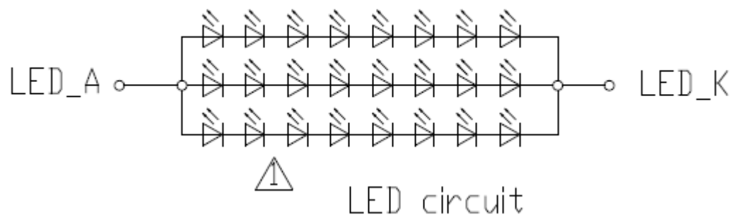
Figure5.2 LED connection of backlight
