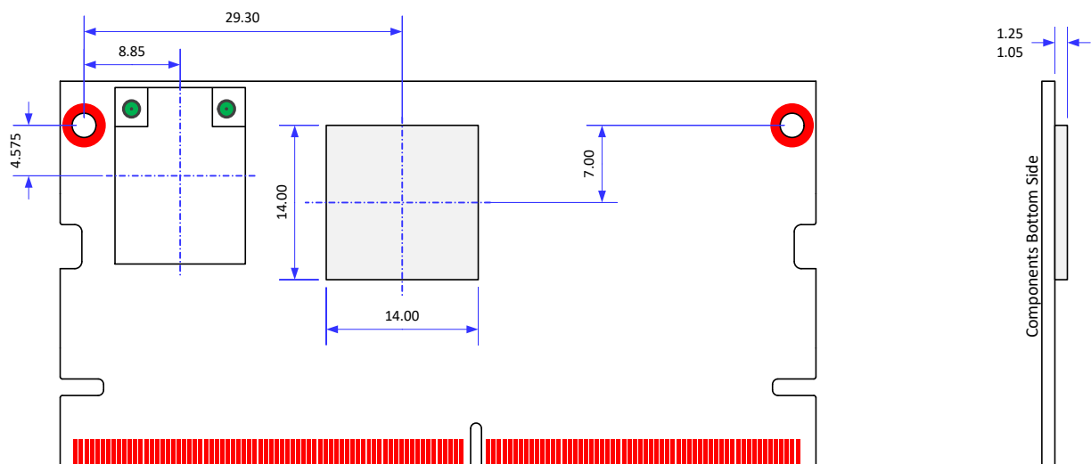
Figure 15 Mechanical position of i.MX 8MM SoC (top view) Tolerance for all measures: \pm 0.1\text{mm} , unless otherwise specified
