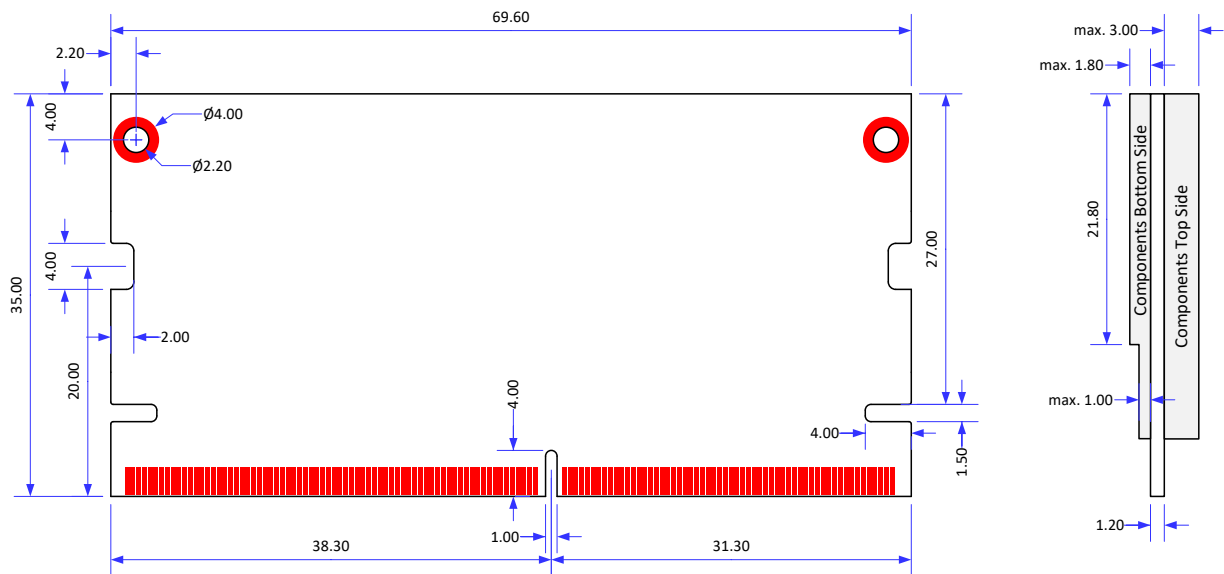
Figure 14 Mechanical dimensions of the Verdin module (top view) Tolerance for all measures: \pm 0.1\text{mm} , unless otherwise specified
