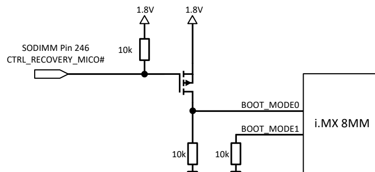
Figure 13: Recovery Mode Circuit
